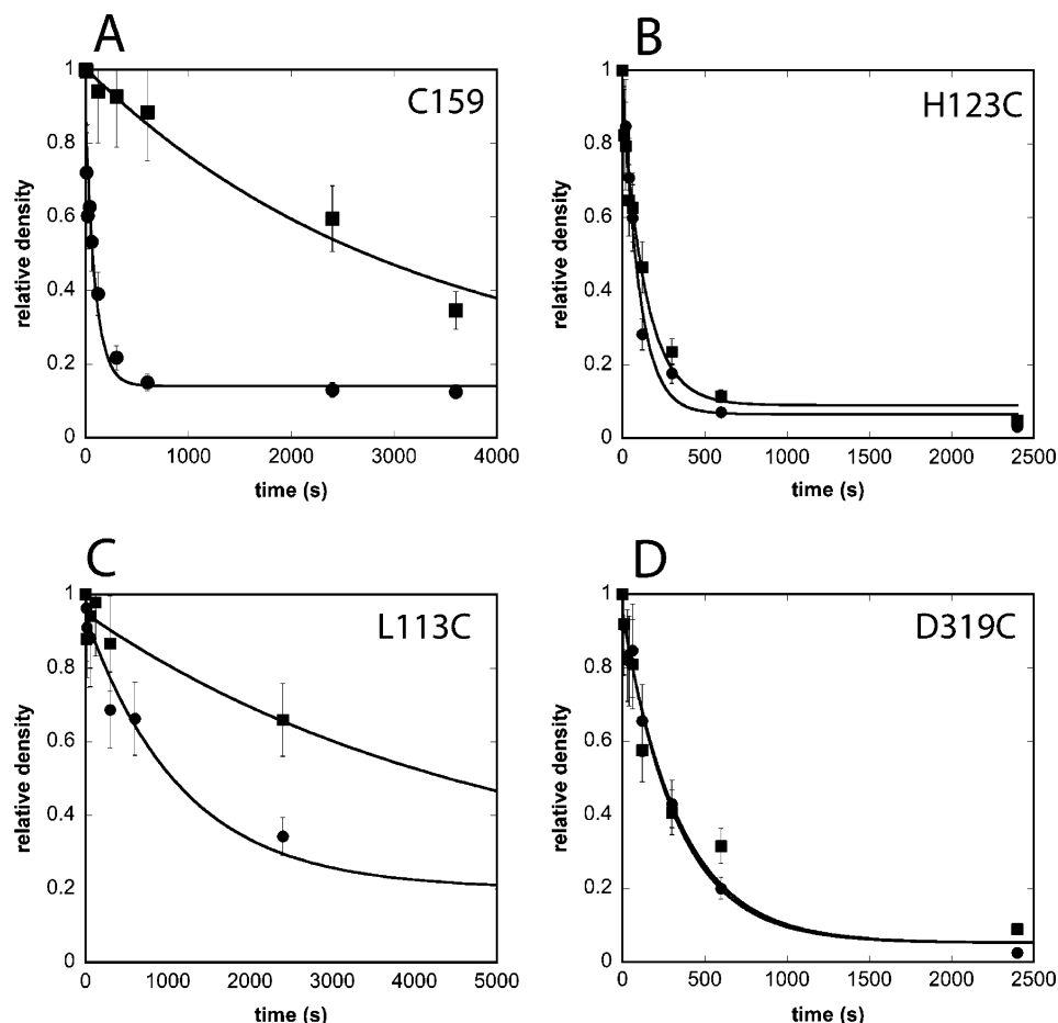
FIGURE 7: Alkylation of ERK2-CTs versus time in the presence and absence of a D-site peptide. Representative plots (A–D) showing the time course for the disappearance of unalkylated ERK2-CTs (measured by the presence of NTCB-mediated cleavage product) in the presence (●) and absence (■) of 0.625 mM of peptide QKGRKPRDLELPLSPSL. The relative density of each gel quadrant (reproducible to within 20% after normalizing for variability in background radioactivity) containing a band associated with the ERK2-CT cleavage product was determined at various time points by phosphorimage analysis of gels similar to those shown in Figure 6 (see Experimental Procedures). The line through the data corresponds to the best fit to a first-order rate law (reproducible to within 30%). Endpoints used to determine rate constants for each alkylation reaction were determined after more than 10 half-lives. Some variability in the relative densities of the endpoints is seen between experiments, which mainly reflect variability in the background radioactivity of the gel quadrants used to determine the relative densities. Replicate experiments were performed on a minimum of two different preparations of each ERK2-CT. The sensitivity and reproducibility of the footprinting analysis are such that a 2-fold difference in a rate constant for alkylation may be readily determined. Rate constants and errors are reported in Table 1.
