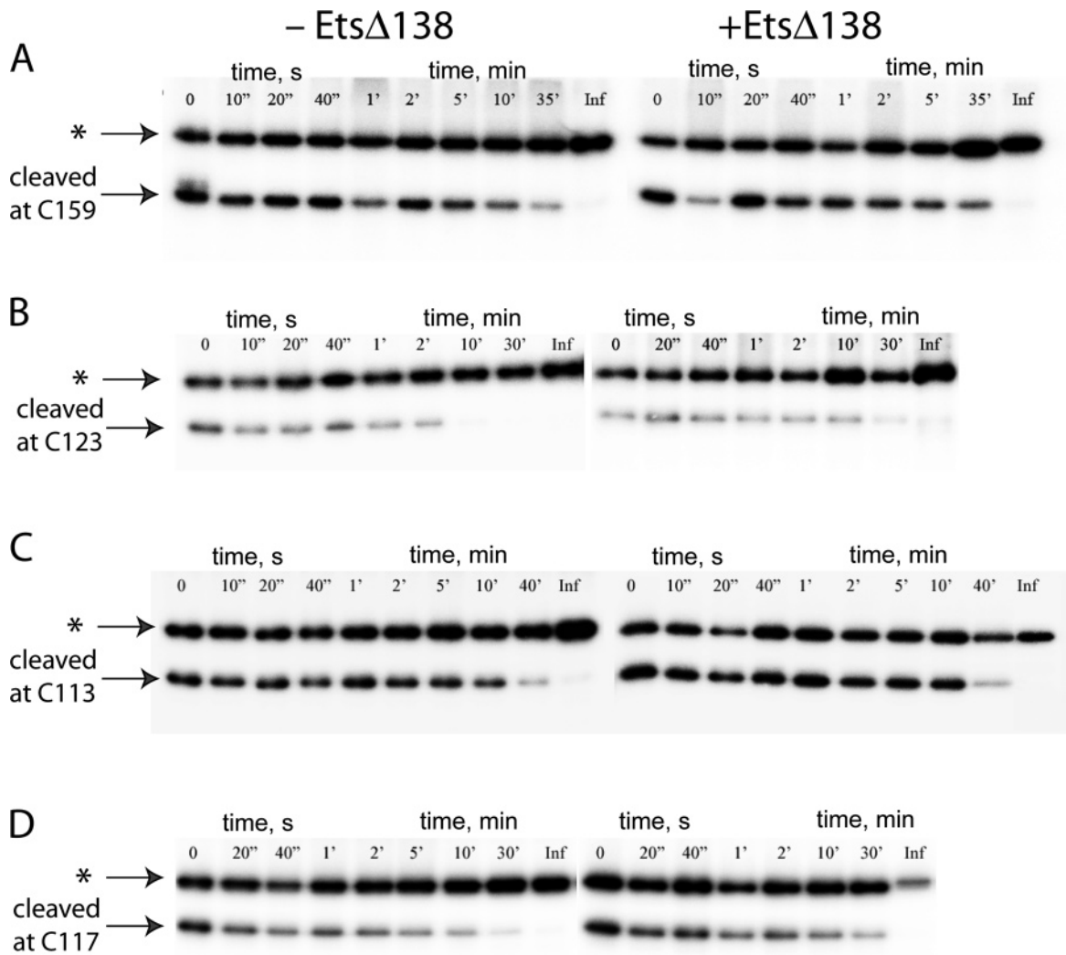
FIGURE 3: Cysteine footprinting of the ERK2 and EtsΔ138-ERK2 complexes. C-terminally radiolabeled single cysteine ERK2 mutants (A, C159; B, H123C; C, L113C; and D, Q117C) were alkylated by iodoacetamide at pH 8.3 and 23 °C in the absence and presence of 1.45 mM EtsΔ138. At the times indicated above each lane, 30 μL aliquots were quenched with excess DTT, and the ERK2 was separated from excess EtsΔ138 (where necessary), denatured, and then cyanylated with excess (25 mM) 2-nitro-5-thiocyanobenzoic acid (NTCB). The cyanylated proteins were precipitated, washed, then resuspended and cleaved in 0.6 M NH 4 OH. Samples were then fractionated by 15% SDS-PAGE, the gels dried, and the bands quantified on a Phosphorimager (see Experimental Procedures). The lanes correspond to the time when an aliquot was quenched. The upper band corresponds to uncleaved ERK2 (see II and III in Scheme 2), and the lower band corresponds to the fragment C-terminal to the single cysteine ( IV in Scheme 2).
