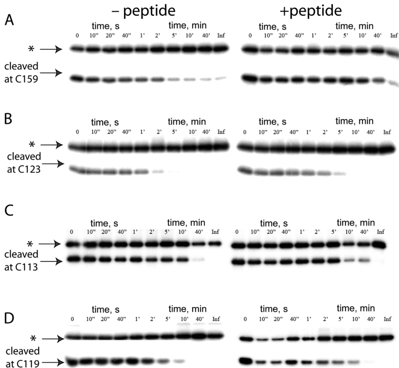
FIGURE 6: Cysteine footprinting of a peptide-ERK2 complex. C-terminally radiolabeled single cysteine ERK2 mutants (A, C159; B, H123C; C, L113C; and D, L119C) were alkylated by iodoacetamide at pH 8.3 and 23 °C in the absence and presence of 0.625 mM peptide; QKGRKPRDLEPLPSL. At the times indicated above each lane, 30 \mu L aliquots were quenched with excess DTT and the ERK2 was separated from excess Ets \Delta 138 (where necessary), denatured, and then cyanylated with excess (25 mM) 2-nitro-5-thiocyanobenzoic acid (NTCB). The cyanylated proteins were precipitated, washed, then resuspended and cleaved in 0.6 M \text{NH}_4\text{OH} . Samples were then fractionated by 15% SDS-PAGE, the gels dried, and the bands quantified on a Phosphorimager (see Experimental Procedures). The lanes correspond to the time when an aliquot was taken. The upper band corresponds to unalkylated ERK2 (see II and III in Scheme 2), and the lower band corresponds to the fragment C-terminal to the single cysteine ( IV in Scheme 2).
