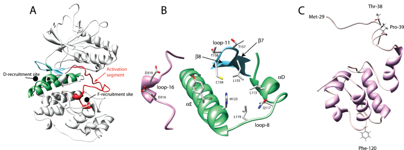
FIGURE 1: Structure of Ets \Delta 138 and ERK2. A. Ribbon diagram of activated ERK2 (PDB 4ERK) showing the D-recruitment site (DRS) and the F-recruitment site (FRS). The activation segment ( 165 DFG–APE 195 ) is colored red. B. The DRS of ERK2 is composed of three segments: segment 1, helix \alpha D–loop-8–helix \alpha E (green); segment 2, strand \beta 7–loop-11–strand \beta 8 (cyan); and segment 3, loop-16 which contains the CD-site (Asp-316 and Asp-319) (plum). Several amino acids that have been shown to be important for recognition of various ERK2 ligands are indicated. C. A ribbon diagram depicting the NMR structure of Ets-1 (29–138) (PDB 1BQV) showing Thr-38 and Pro-39 in the flexible N-terminal tail, as well as Phe-120 in the PNT domain.
