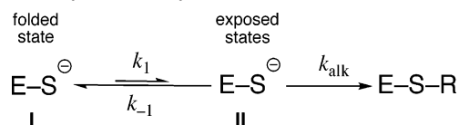
Scheme 1: Model Describing an Equilibrium between the Folded State and Unfolded Exposed States That Determines the Rate of Cysteine Alkylation
