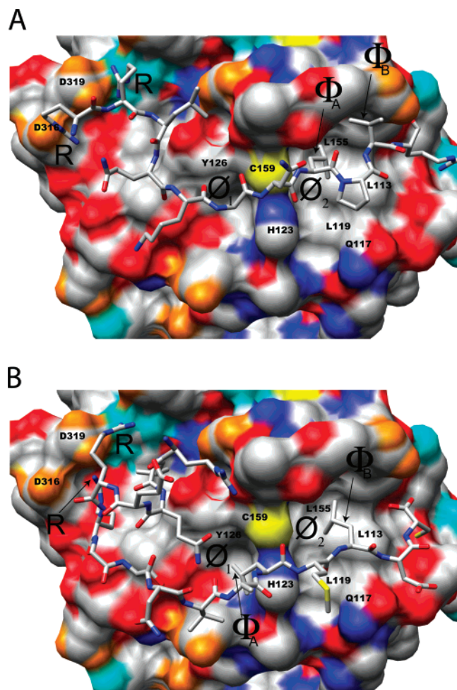
FIGURE 2: Differences in the binding modes of D-site peptides to the DRS of ERK2. A. Binding of the D-site peptide RRLKQGN-LPVR (consensus; (R/K) 2-3 -X 4-6 -Φ A -X-Φ B ) derived from MAP kinase phosphatase-3 to unactivated ERK2. The Φ A residue occupies the hydrophobic site Ø 2 . B. The binding of the D-site peptide RLQERRGSNVALMLDV, derived from hematopoietic protein tyrosine phosphatase, to unactivated ERK2. The Φ A and Φ B residues of hematopoietic protein tyrosine phosphatase occupy the hydrophobic Ø 1 and Ø 2 sites, respectively. Surface representations: red, oxygen; orange, carboxylate oxygen; blue, neutral nitrogen; cyan, ε lysine nitrogen, or arginine guanidino nitrogen.
